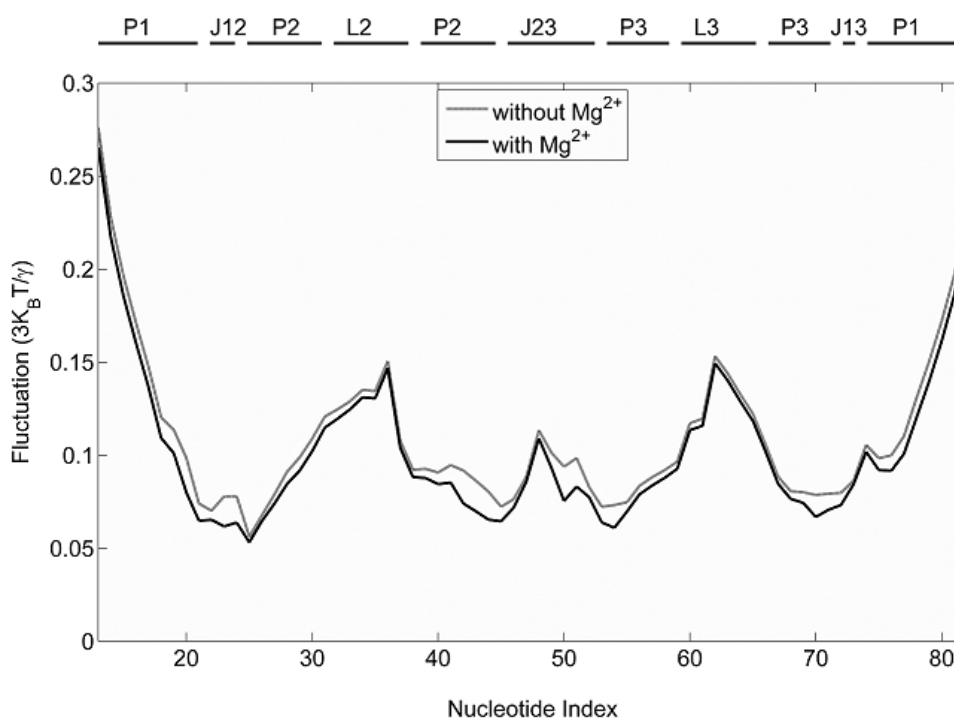
Figure S1. Fluctuations of nucleotides of add A-riboswitch with (solid line) and without Mg^{2+} ions (shaded line), respectively.
